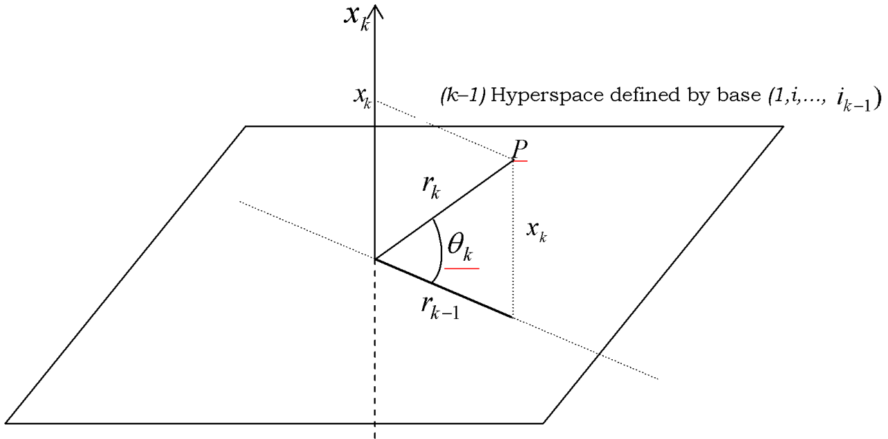
Figure 11.1: Hyperspherical coordinates
