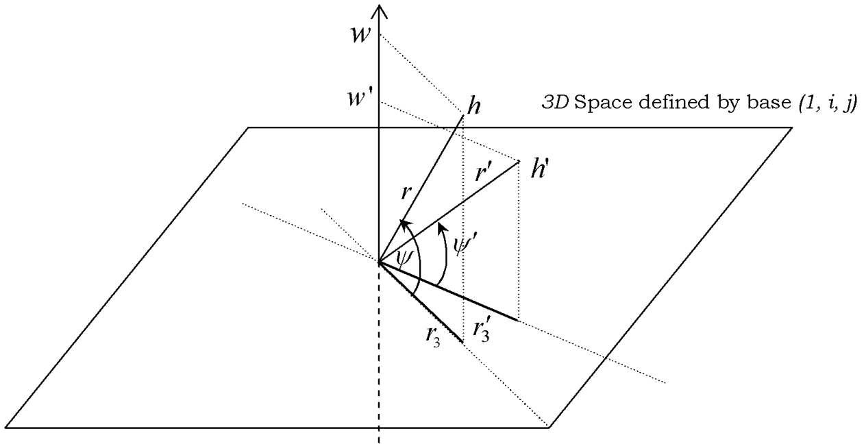
Figure 11.2: Four dimensional hypercomplex multiplication
