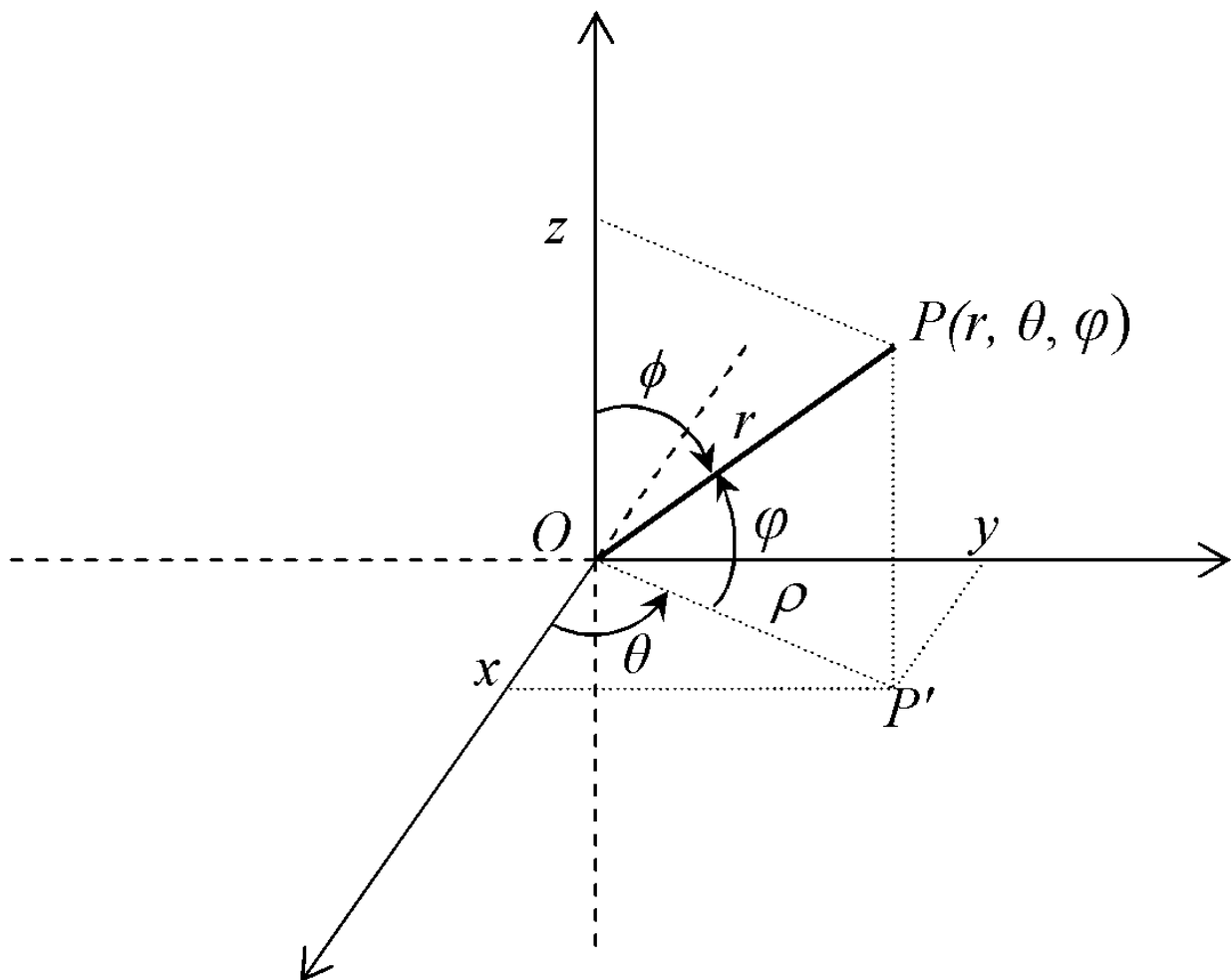
Figure 3.1: Spherical coordinates
