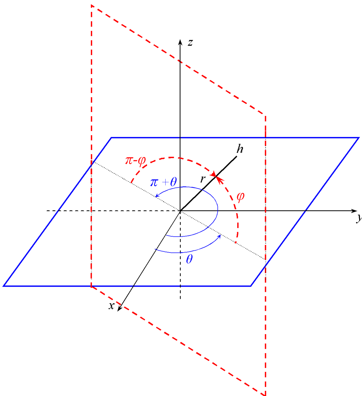
Figure 4.1: Duplicity or duplication/replication of 3D spherical hypercomplex numbers
