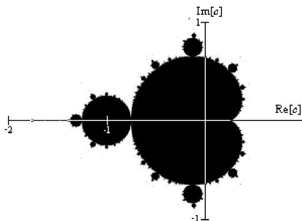
Figure 13.1: Mandelbrot set. 16
