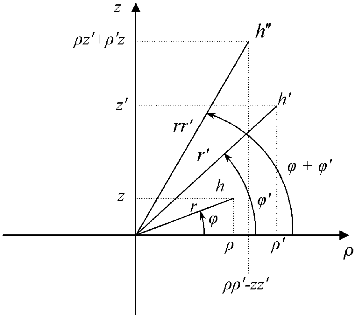
Figure 3.3: Multiplication in the orthogonal planes containing Oz
