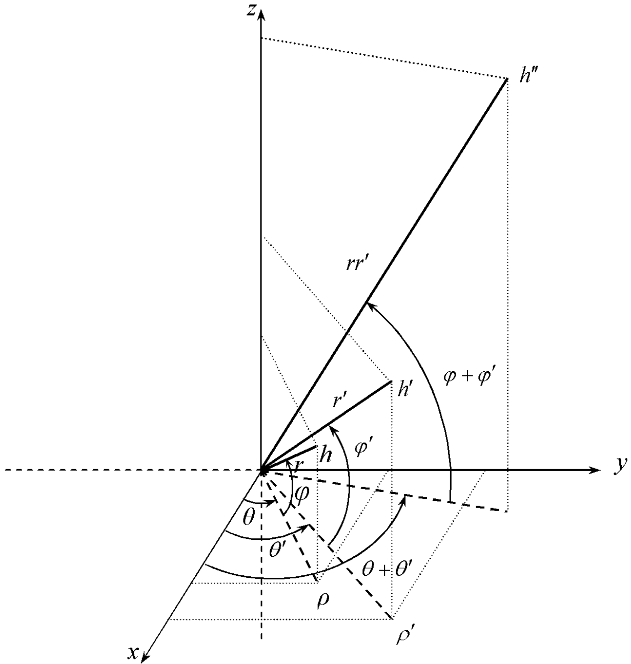
Figure 3.2: Multiplication of two triples h and h' .
