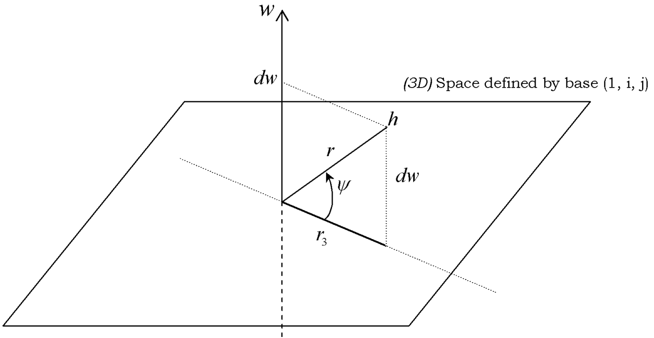
Figure 13.4: Minkowski space and 4D hyperspherical hypercomplex numbers
